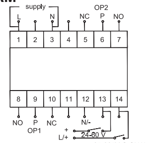
PANEL / FLUSH MOUNT
